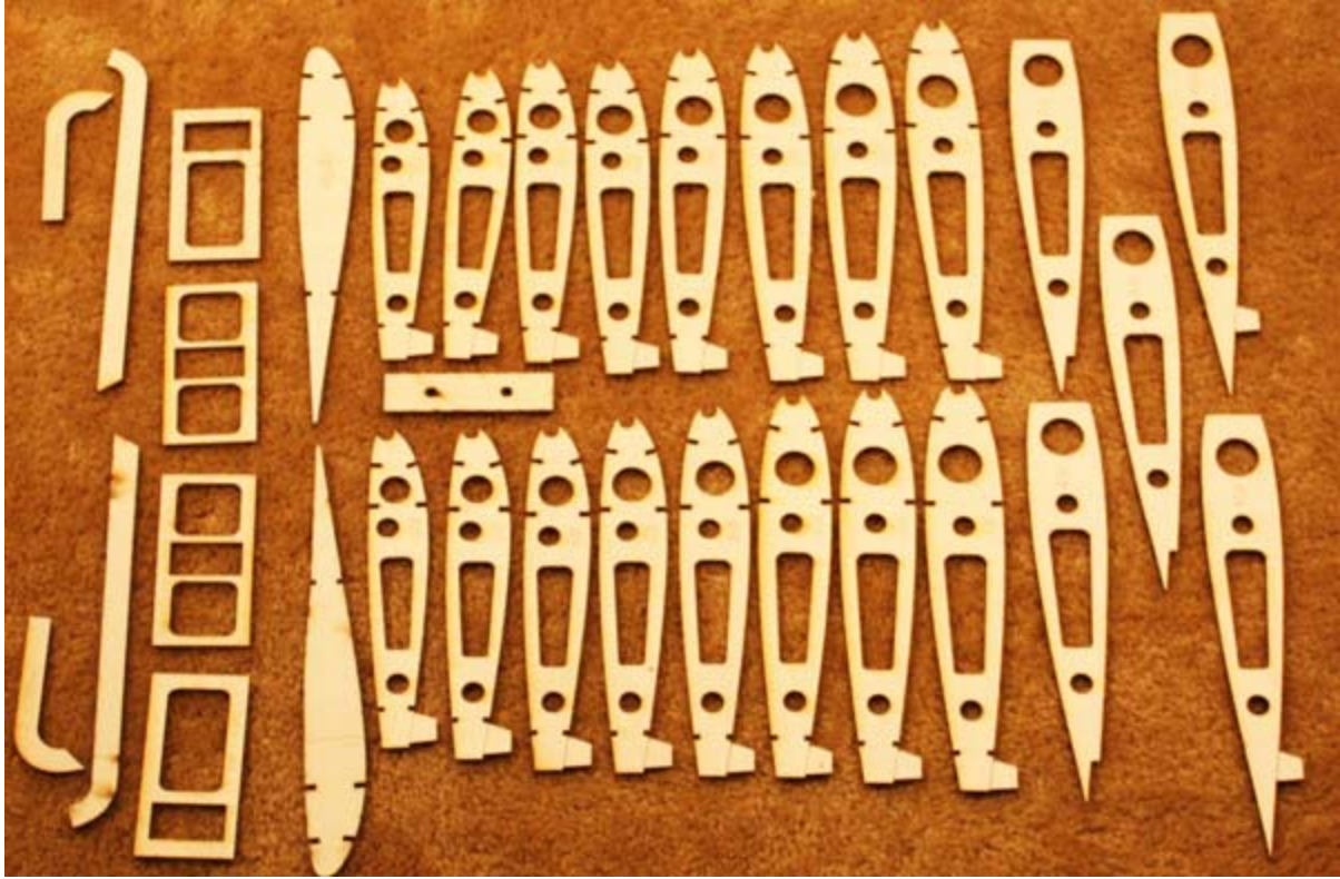
A preformed aluminum main gear is available, as is a laser-cut short kit with either or both wing options from Creative Hobbies. Full-size plans are available at the end of this article. Source information for these and other building materials can be found at the end of this article.
