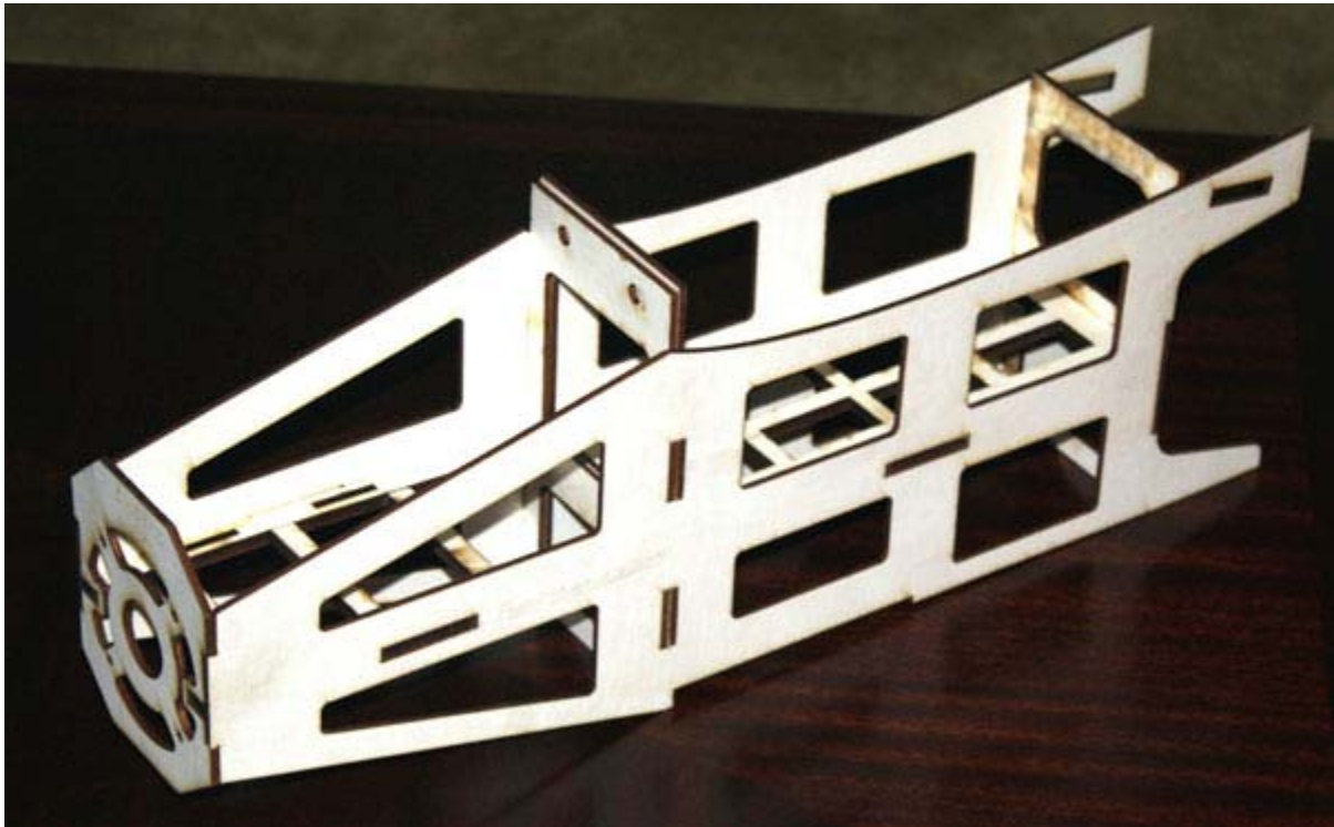
A preformed aluminum main gear is available, as is a laser-cut short kit with either or both wing options from Creative Hobbies. Full-size plans are available at the end of this article. Source information for these and other building materials can be found at the end of this article.
